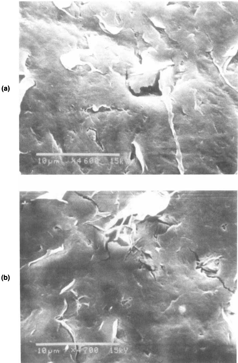
FIGURE 7 SEM of (a) original skived PTFE surface (b) DDM-primed PTFE surface.
