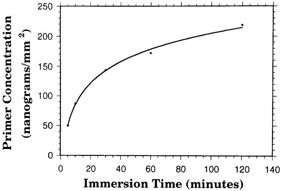
FIGURE 1 TPP surface concentration as a function of immersion time in molten primer at 120°C.
