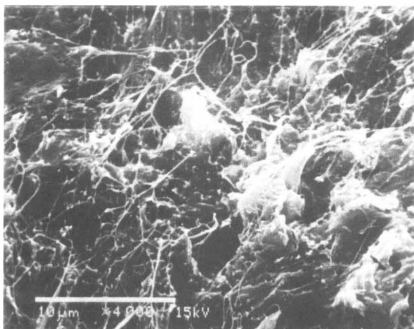
FIGURE 6 SEM of fracture surface of PTFE/Epoxy adhesive bond showing (a) interfacial (b) cohesive failure in the PTFE.
