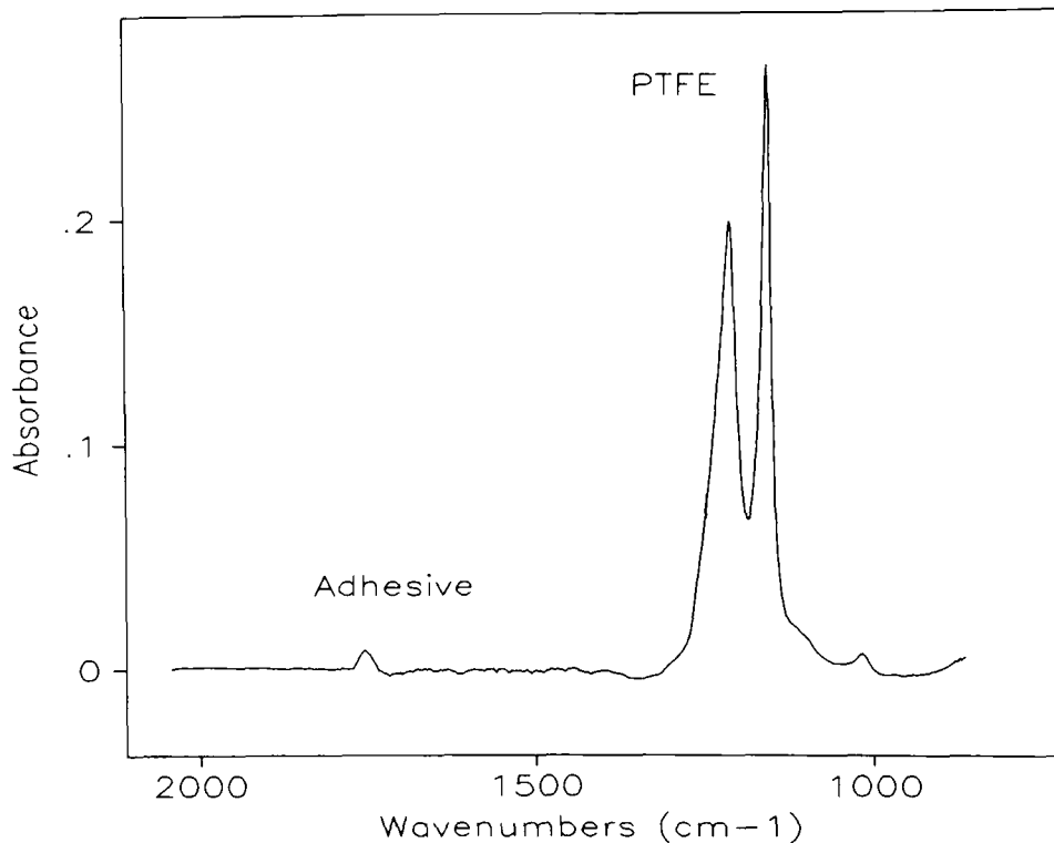
FIGURE 4 IR-IRS spectrum (germanium element, 60-degree incidence) or nitromethane-washed model adhesive bond.
