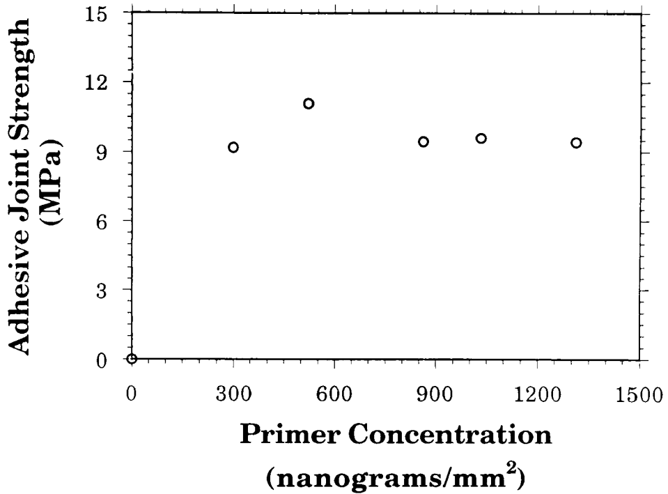
FIGURE 2 Adhesive bond strength as a function of TPP primer surface concentration.
