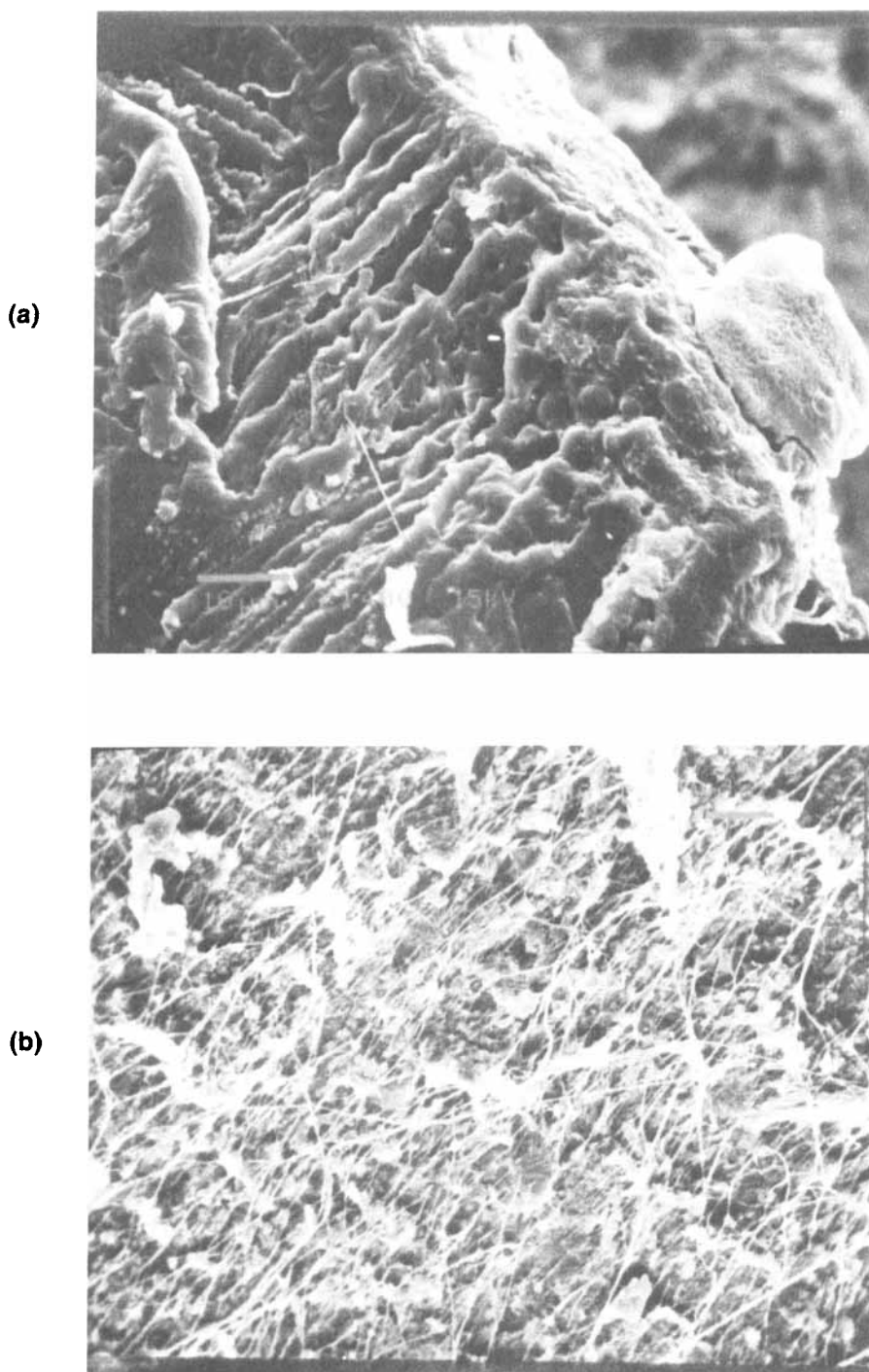
FIGURE 3 SEM of fracture surface of PTFE/CA adhesive bond showing (a) cohesive failure in CA (b) cohesive failure in PTFE.
