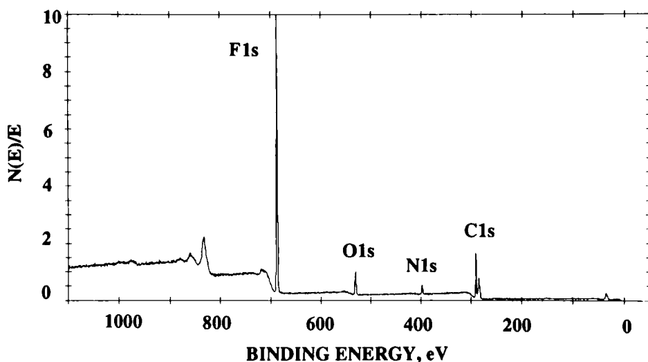
FIGURE 5 XPS spectrum of nitromethane-washed model adhesive bond.
